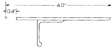
Fig. 7 Redhawk spoiler cross section.
