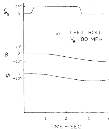
Fig. 10 Roll time histories for the Redhawk.
