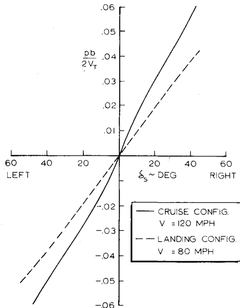
Fig. 9 Steady-state roll helix angle with spoilers.
