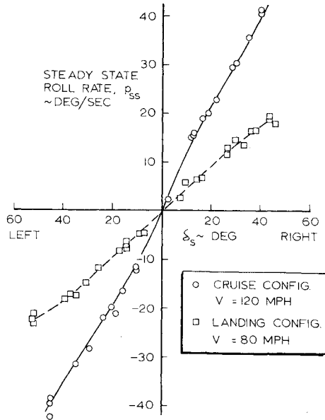
Fig. 8 Redhawk spoiler roll rate data.
