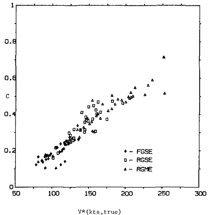
Fig. 3 Cruise Efficiency C (eqn. 6) vs. Cruise Optimum (true) Airspeed, 111 Piston Aircraft.
